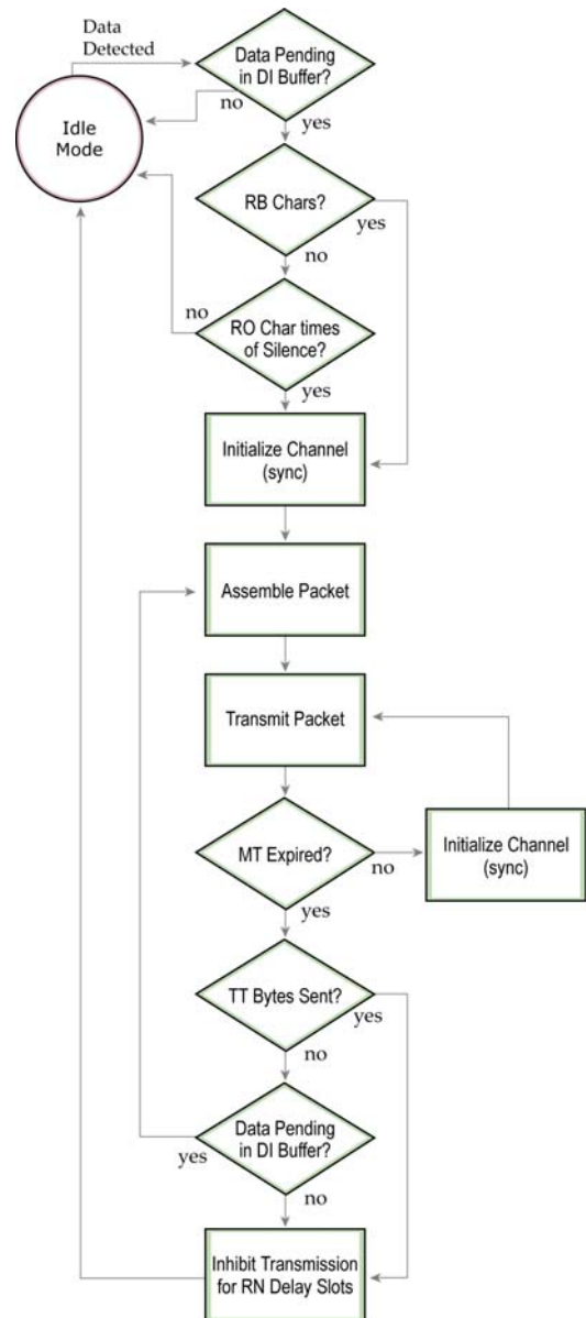
Figure 4-05. Multi-Transmit Mode State Diagram (TX Module)
